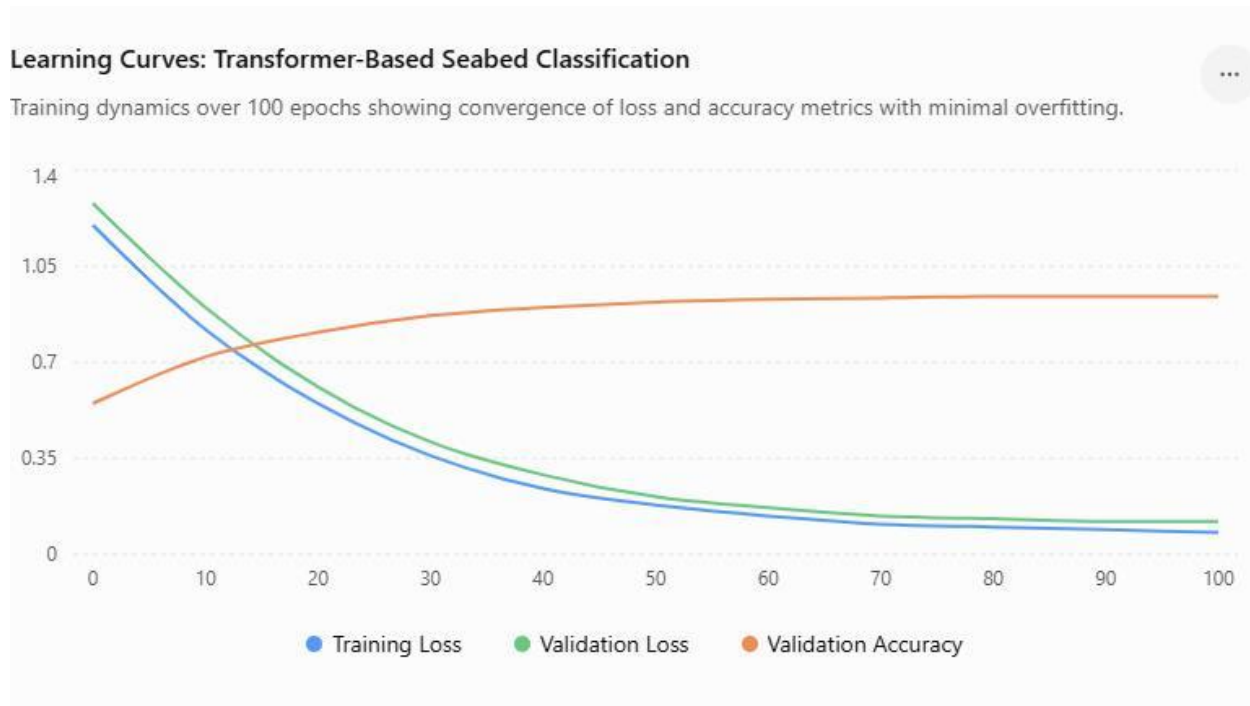
Figure 10. Training and validation loss/accuracy curves over 100 epochs for a transformer-based seabed classification model
